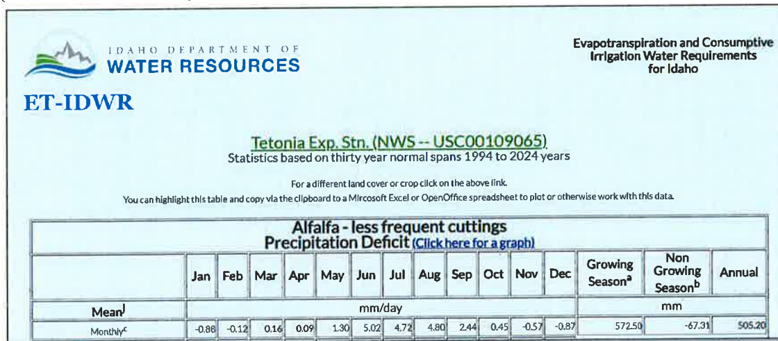
Figure 1. ET Values for –Alfalfa – Less Frequent Cuttings at Tetonia Experiment Station (NWS – USC00109065).
