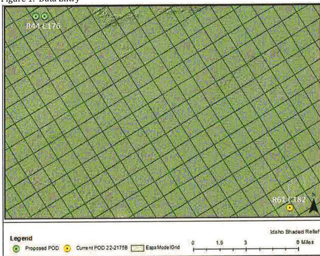
Figure 1. Data Entry
