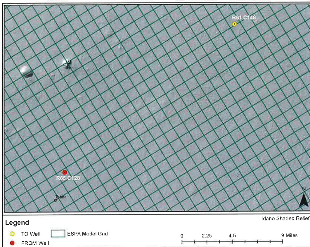
Figure 1. Data Entry
