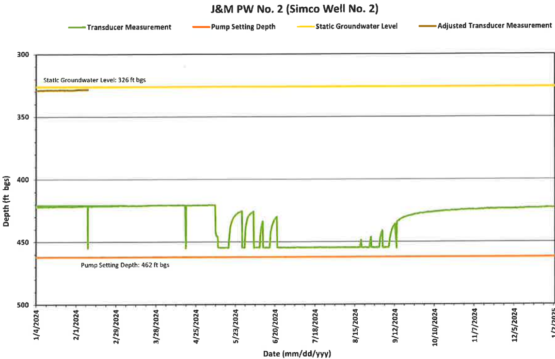
Figure 3-2: Transducer record for well J&M PW No. 2, 2024.
