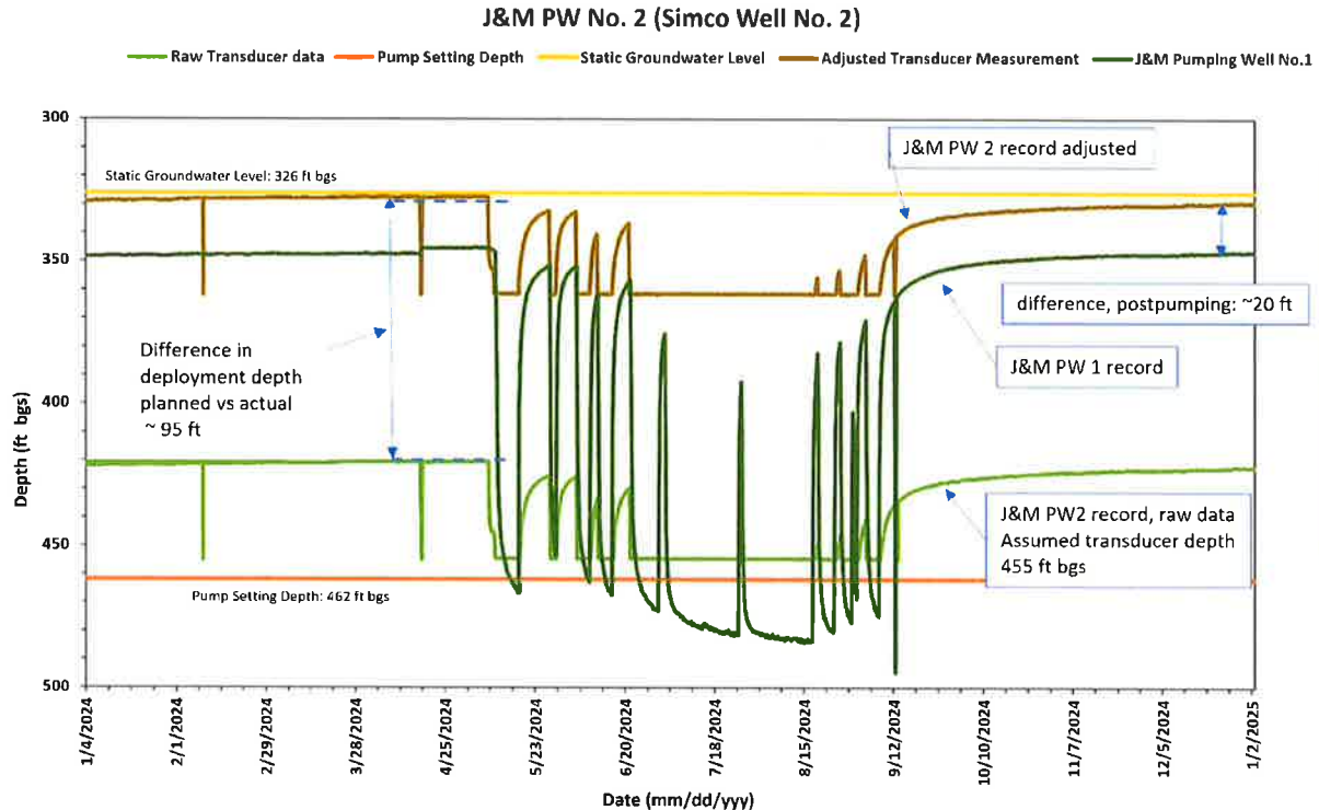
Figure 3-3: J&M PW No. 2 Groundwater Monitoring, with comparative record for J&M PW No.1 and raw and adjusted record for J&M PW No. 2, 2024.
