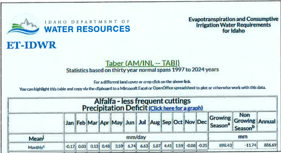
Figure 3. ET Values for Alfalfa – less frequent cuttings at Taber (AM/INL - TABI), obtained on January 2, 2026.
