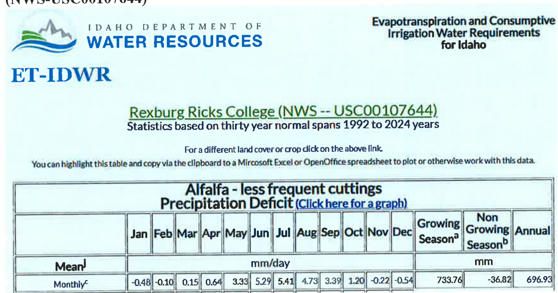
Figure 1. ET Values for Alfalfa – less frequent cuttings at Rexburg Ricks College (NWS-USC00107644)
