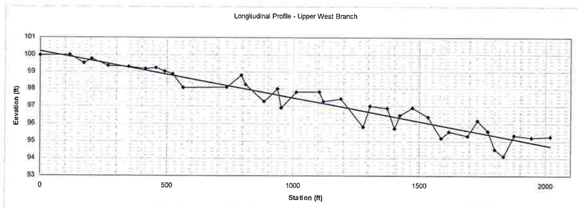
Figure 26. Longitudinal profile of Upper West Branch reference reach.
