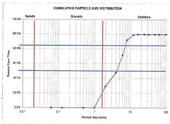
XS: D3 Reach: Riffle
