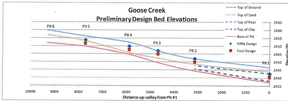
Figure 29. Valley fill stratigraphy and proposed riffle/bed elevations.
