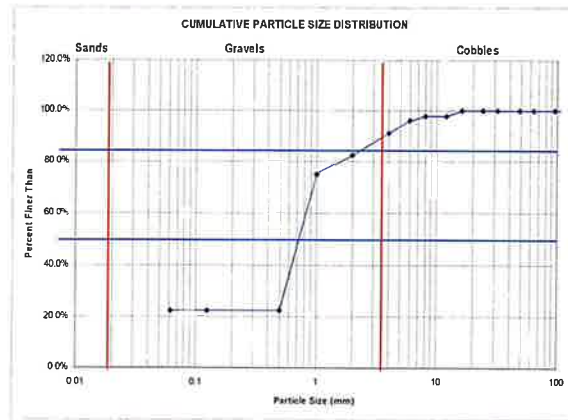
XS: D2 Reach: Pool
