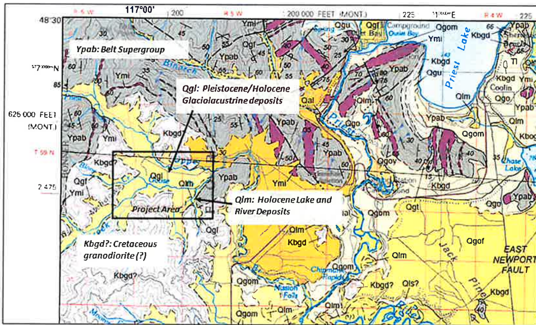
Figure 2. Geologic map of project area (Lewis and others, 2008).
