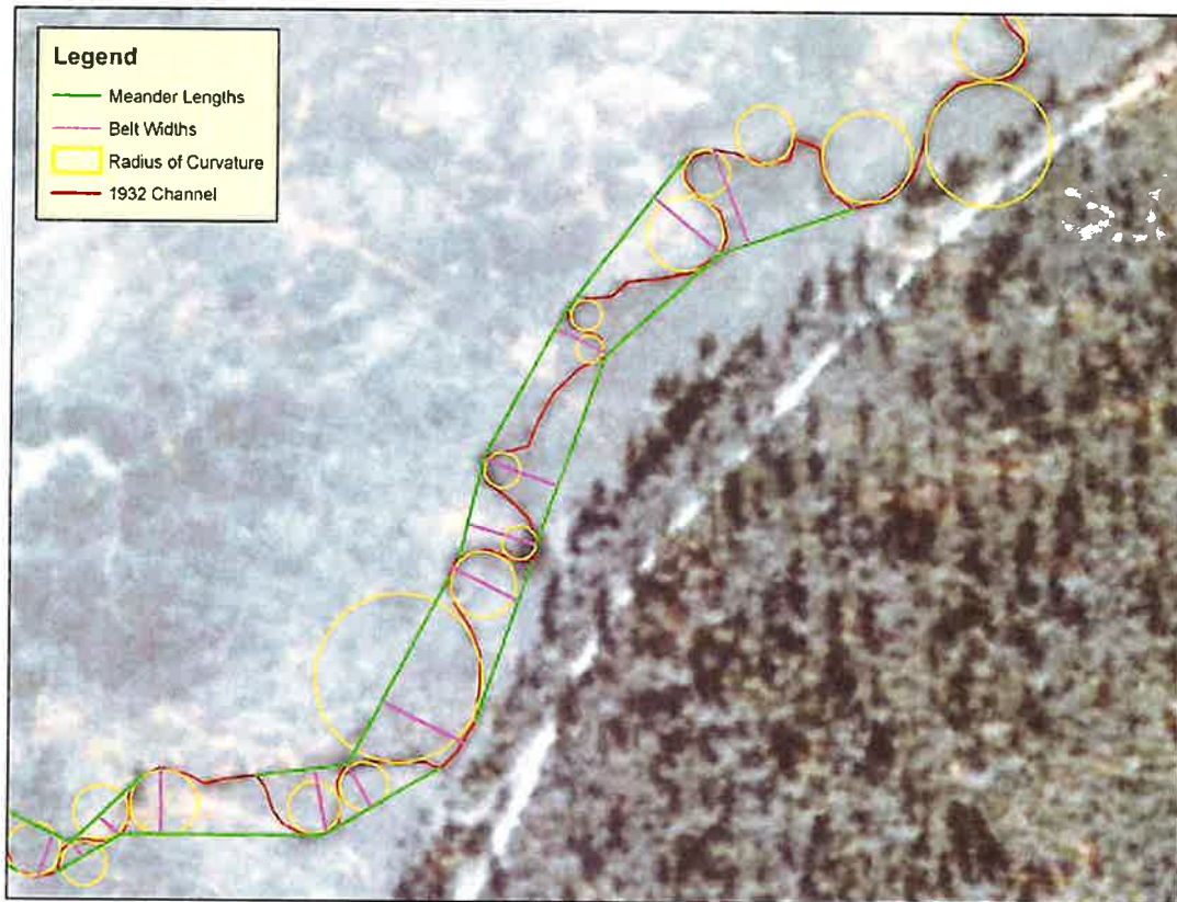
Figure 28. Planform dimensions digitized from 1932 aerials.
