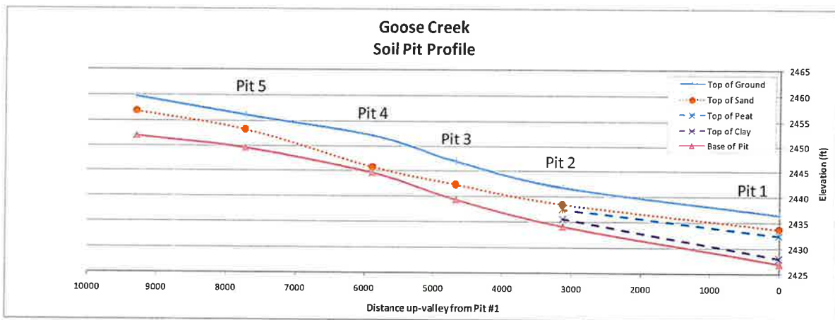
Figure 19. Soil pit profile compiled from pit logs and site elevation survey.
