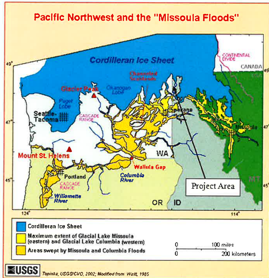
Figure 3. Mapped southern extent of Cordilleran Ice Sheet ( www.USGS.gov ).
