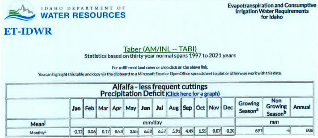
Figure 4. ET Values for Alfalfa – less frequent cuttings at Taber (AM/INL - TABI).
