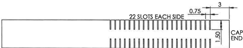
SLOT LAYOUT
