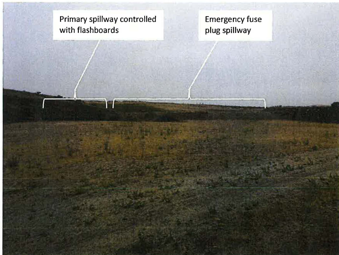
Photo 10: Primary spillway with flashboard controlled entrance and emergency fuse plug spillway.
