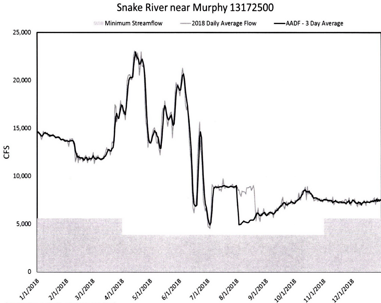
Figure 3. 2018 Average Daily Flow of Snake River below Swan Falls Dam, Adjusted Average Daily Flow (AADF) and Minimum Stream Flow.
