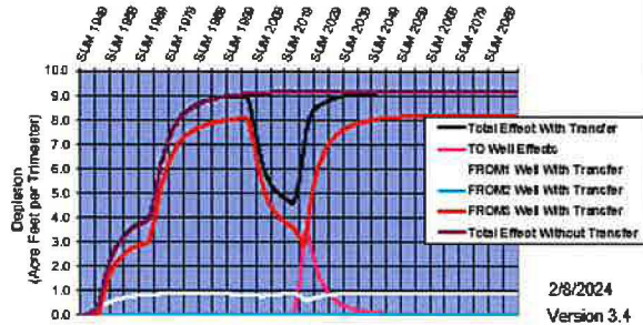
Hydrologic Response—Shelley to Near Blackfoot Customer Name: PEP 3 '22- Transfer No: 0
