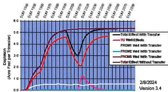
Hydrologic Response—Ashton to Rexburg Customer Name: PEP 3 '22-'24 Transfer No: 0
