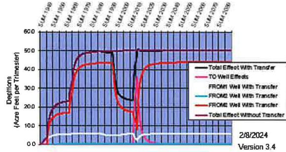
Hydrologic Response—Shelley to Near Blackfoot Customer Name: PEP 3 '22- Transfer No: 0
