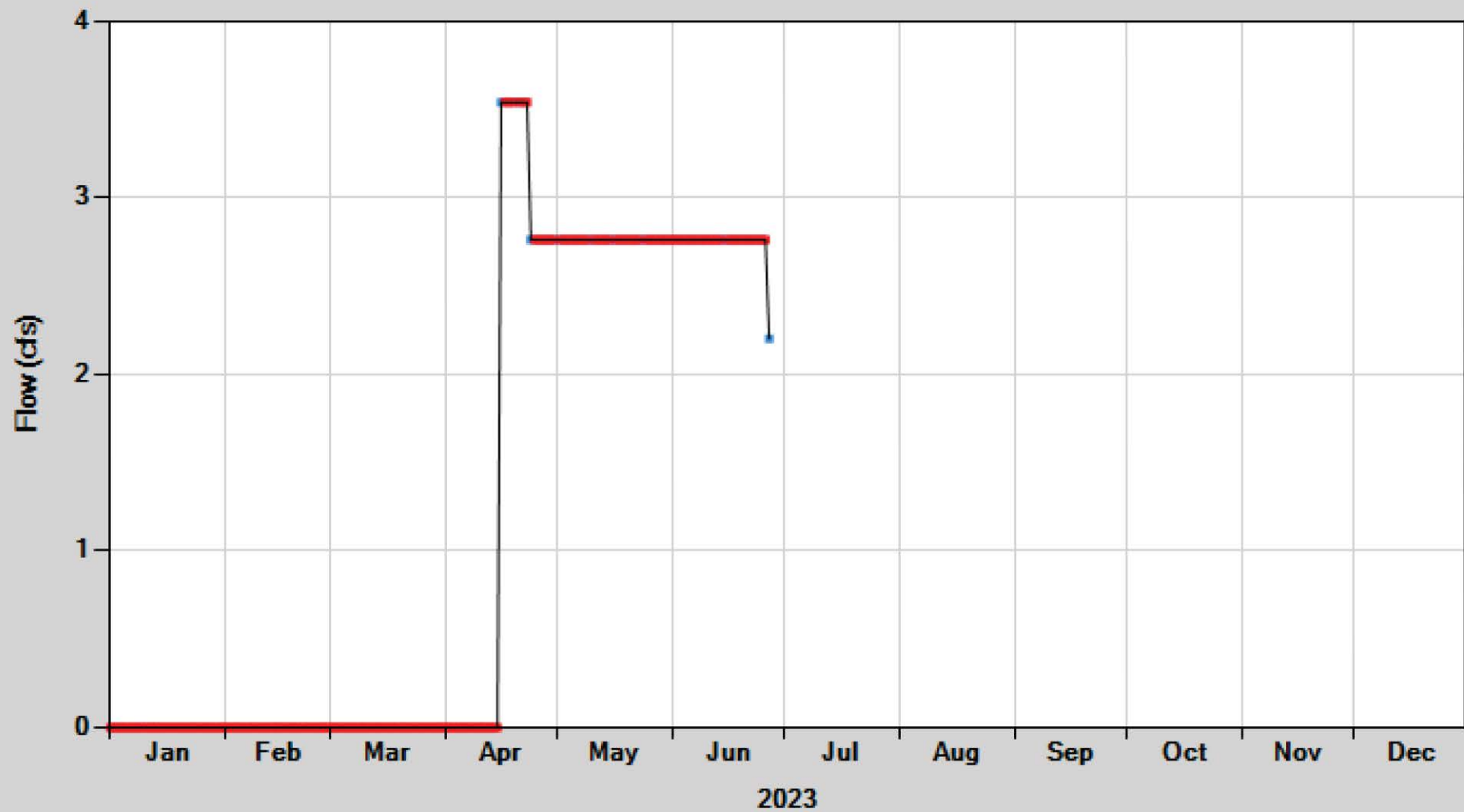
Hydrograph of 119198 - D - 119198
