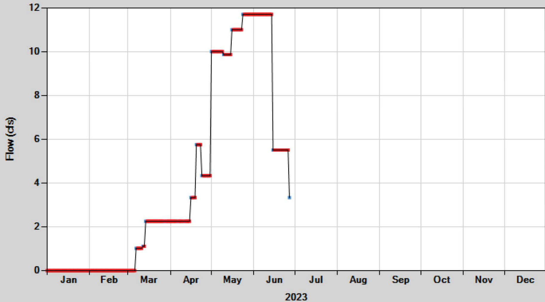
Hydrograph of 119752 - D - 119752
