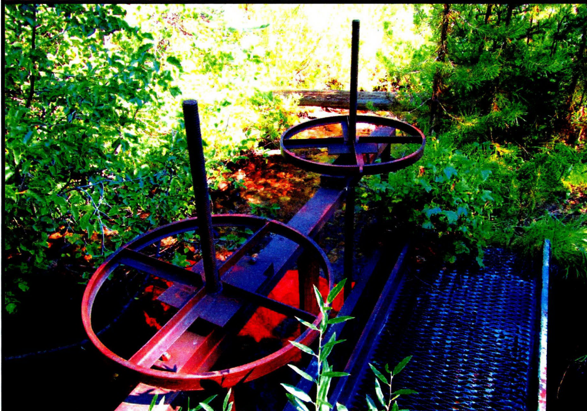
Lockable headgate on Goat Creek 06/07 diversion, 46 meters above fish screen.
