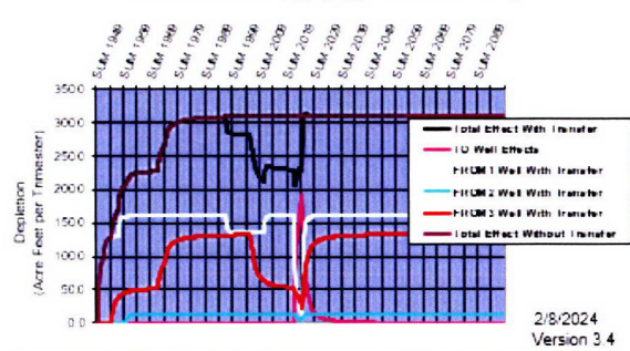
Hydrologic Response-- Neeley to Minidoka Customer Name: PEP 3 '22- Transfer No: 0
