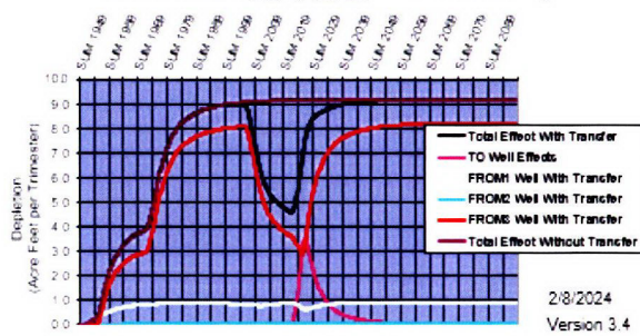
Hydrologic Response--Heise to Shelley Customer Name: PEP 3 '22-'24 Transfer No: 0
