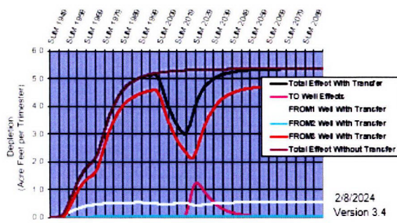
Hydrologic Response--Ashton to Rexburg Customer Name: PEP 3 '22-'24 Transfer No: 0
