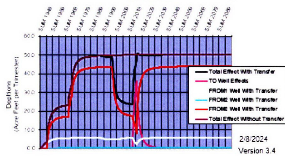
Hydrologic Response--Shelley to Near Blackfoot Customer Name: PEP 3 '22- Transfer No: 0
