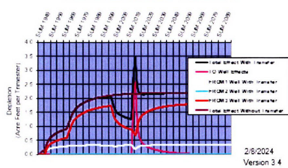
Hydrologic Response-- Neeley to Minidoka Customer Name: PEP 3 '22- Transfer No: 0
