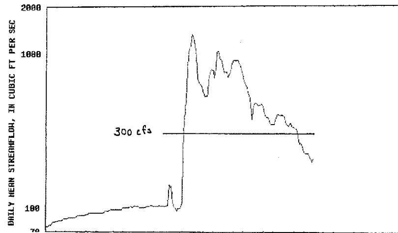
USGS 13132500 BIG LOST RIVER NR ARCO ID
