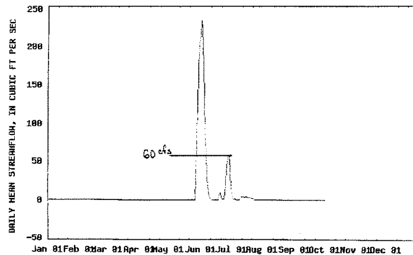
USGS 13132500 BIG LOST RIVER NR ARCO ID
