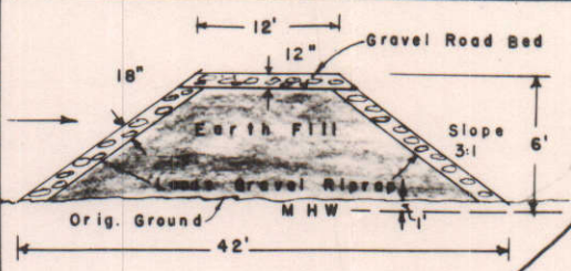
SECTION B-B (SEE PG. 2 OF 2)
