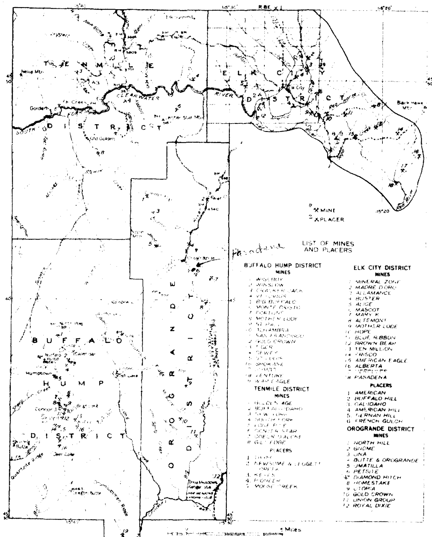
Figure 2.—Map showing locations of mines and veins in the Elk City, Orogrande, Buffalo Hump, and Tennile districts.
