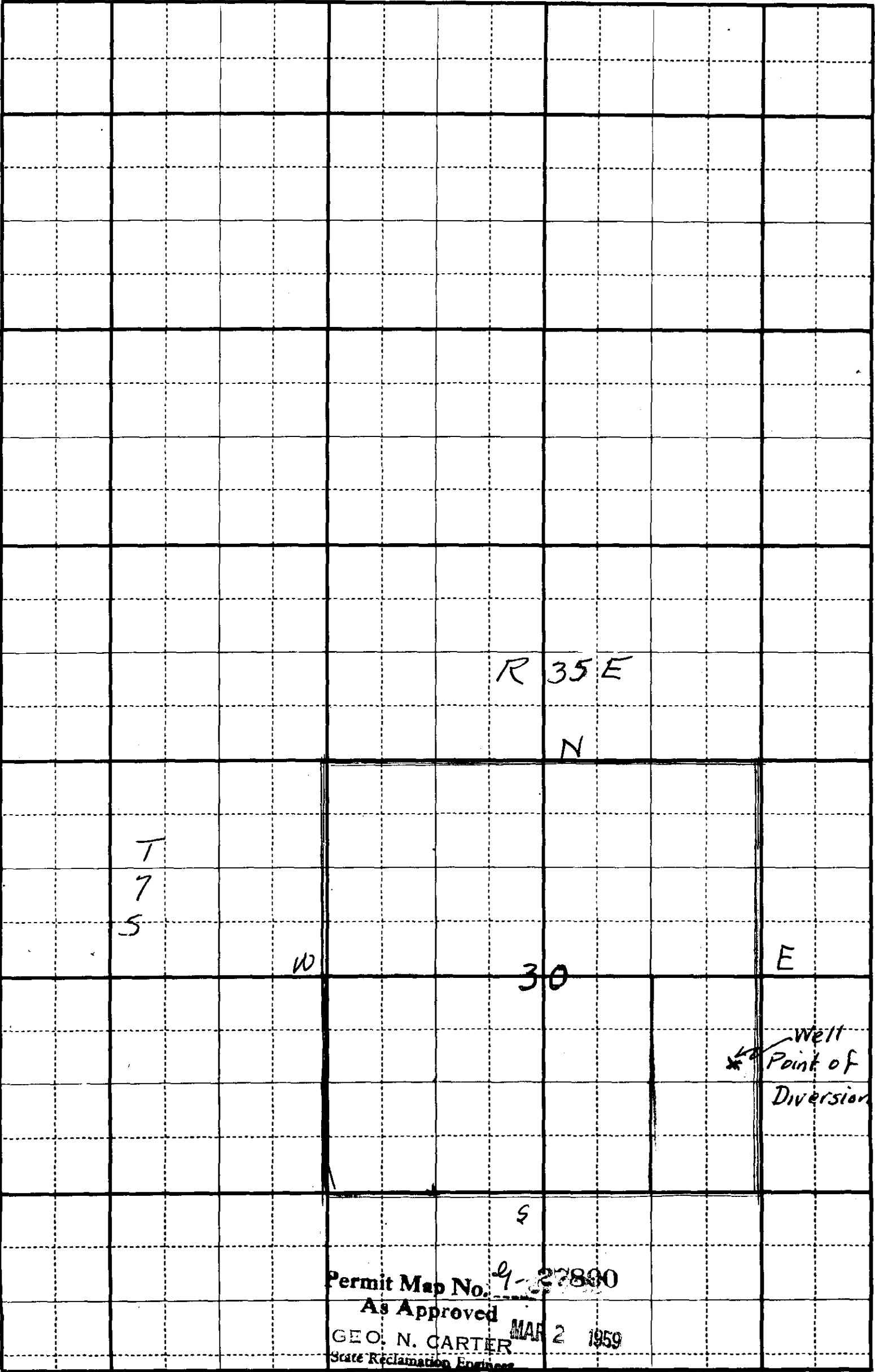
SCALE: 2 Inches Equal 1 Mile. Draw Plan In Ink. Well in SW corner - N 1/4 of E 1/2 SE 1/4 - Sec 30, T 7 S, R 35 - E.B.M. 27800
