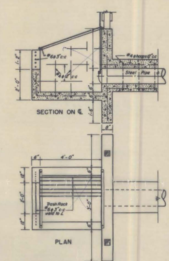
DETAIL OF INTAKE STRUCTURE
