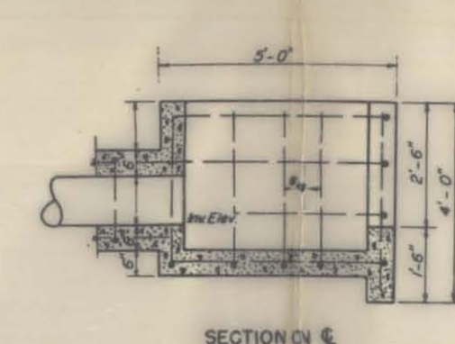
DETAIL OF OUTLET STRUCTURE
