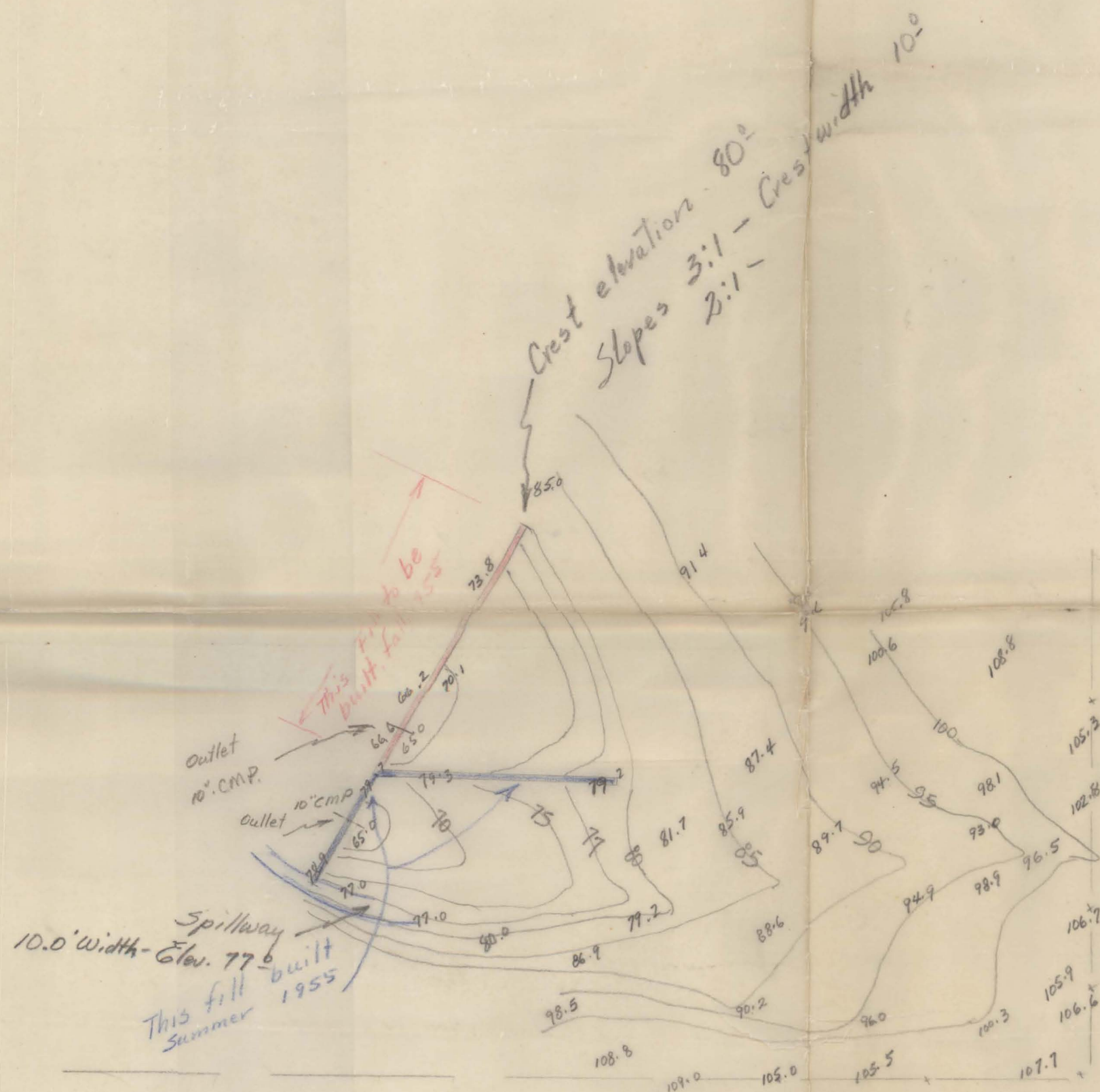
PLAN OF STORAGE AREA AND DAM SITE
