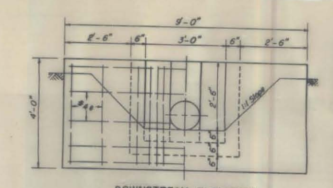
DETAIL OF OUTLET STRUCTURE
