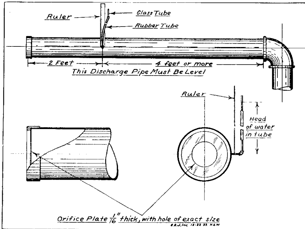
This sketch shows how to construct a Circular Orifice Weir
