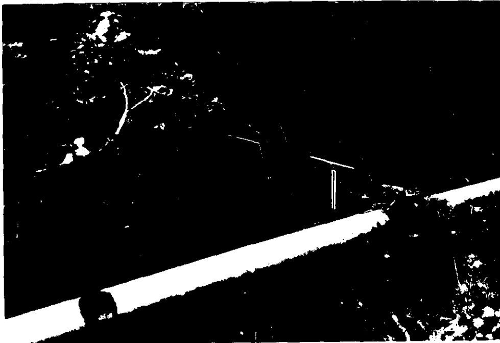
Cippolatti weir (Badger meter is downstream just 20 or 30' on mainline.)
