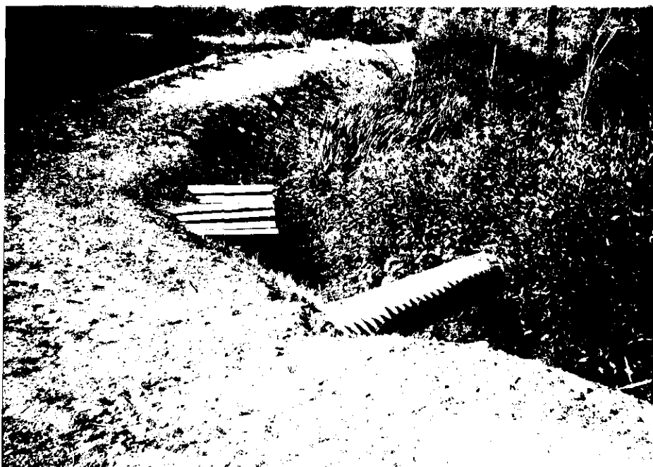
Plate 3 - Overflow culverts (downstream side of dam).
