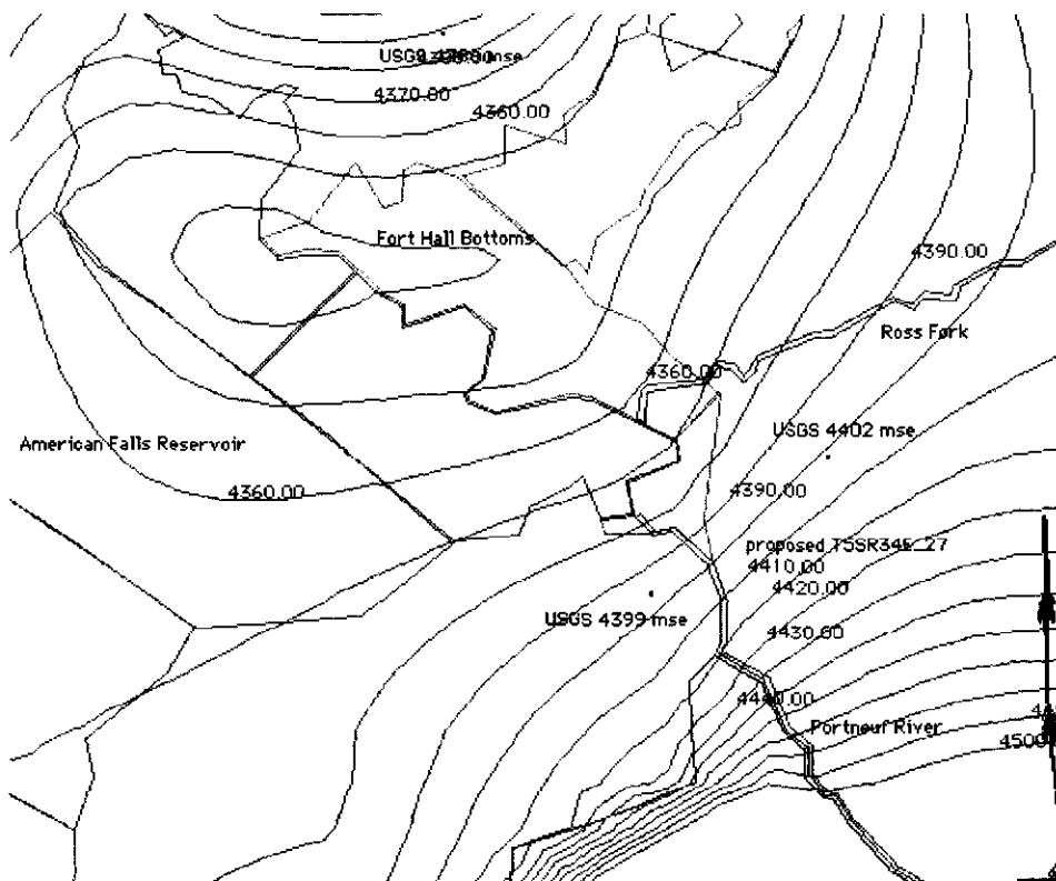
Figure 3. Simulated groundwater elevations and pathlines in the vicinity of proposed well located at T05S R34 E Section 27 NENE.
