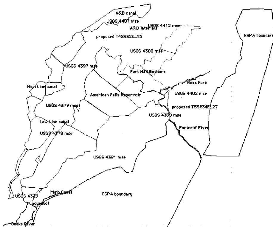
Figure 1. Analytic element model representation of the American Falls area
