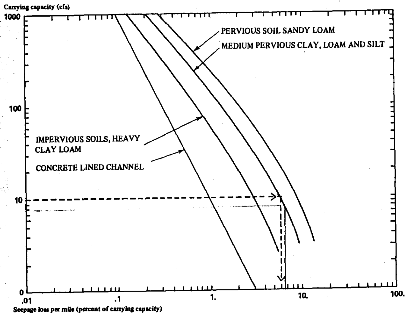
FIGURE 5. Estimating delivery water losses and Moritz formula
