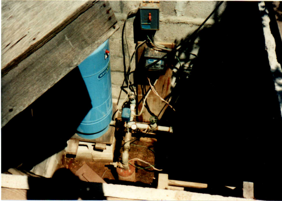
P/D — well & pressure tank
