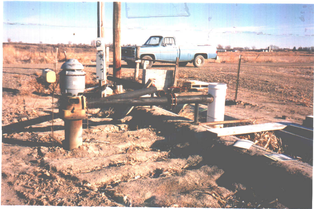
PHOTO ONE- View northerly of well and discharge lines into ditches.
