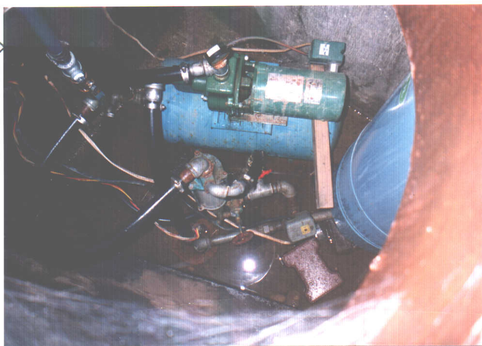
View of the well, motor, pressure tank system underneath well housing
