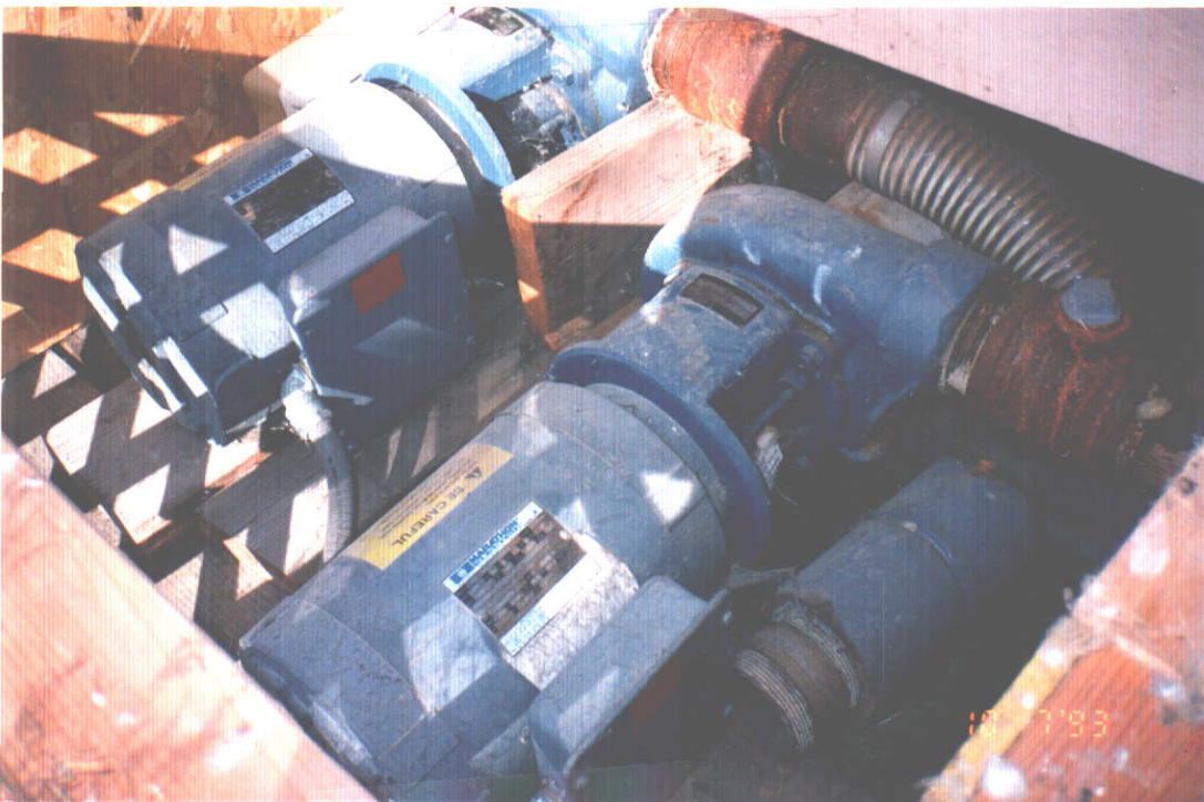
Pump system. Pumps alternate on 12-hr cycles
