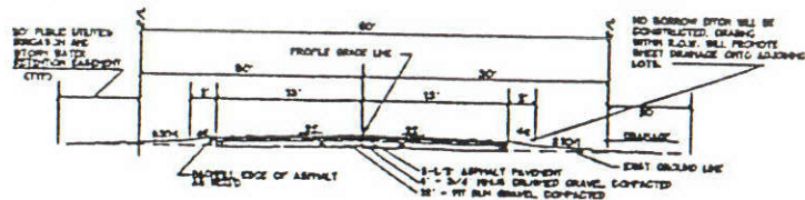
PROPOSED TYPICAL ROADWAY SECTION
