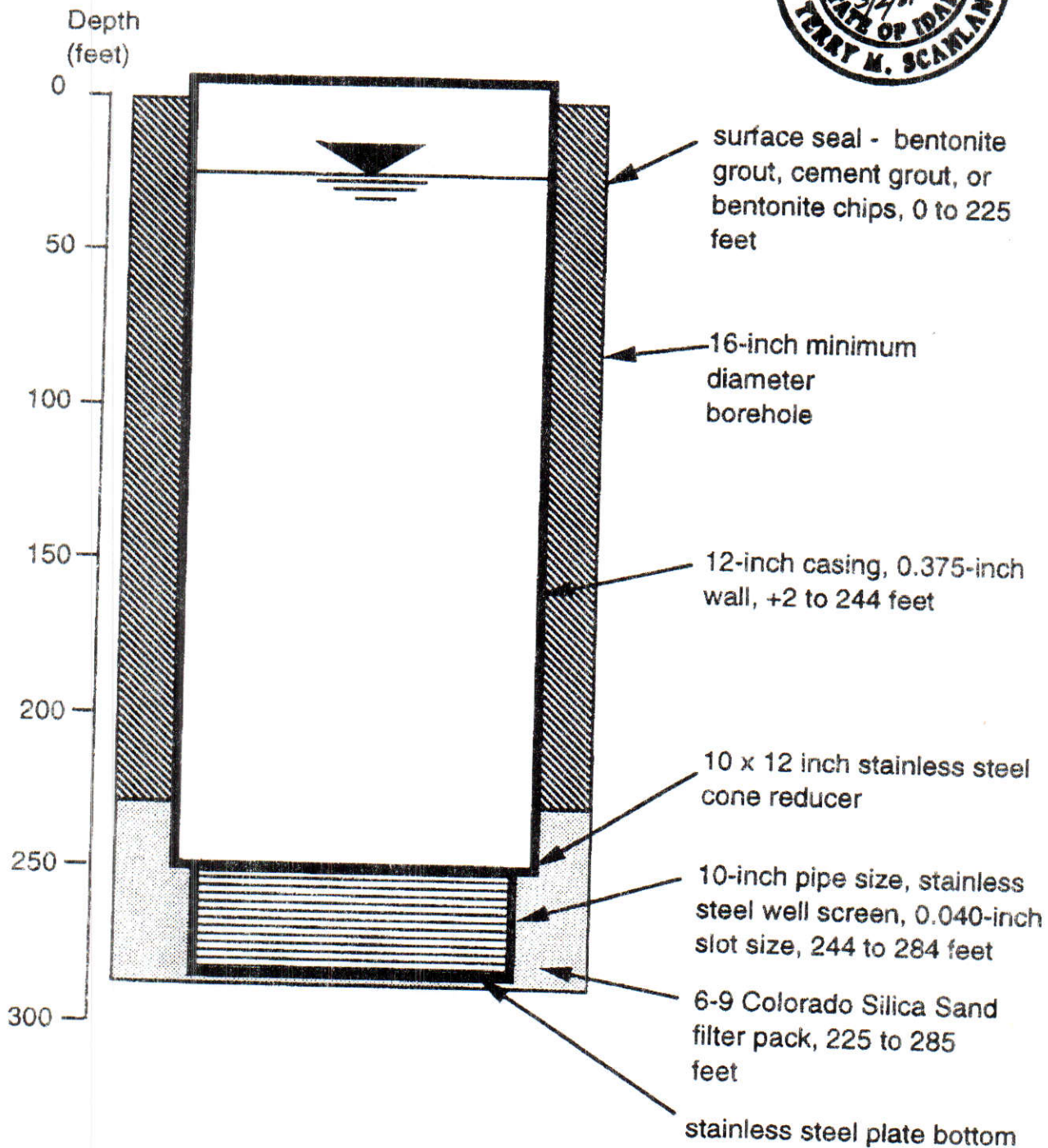
FIGURE 2 - HOMEDALE MUNICIPAL SUPPLY WELL SCHEMATIC
