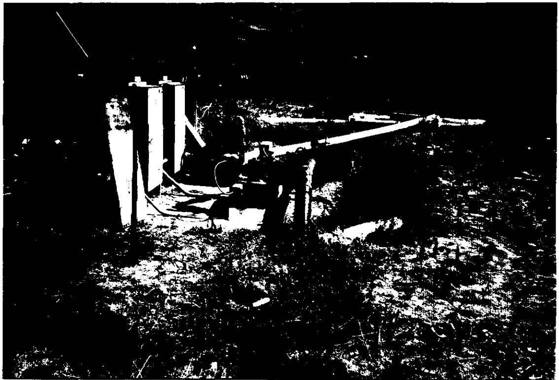
(A) POINT OF DIVERSION TWO SUBMERSIBLE PUMPS ARE SET IN A SINGLE CASING
