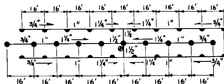
Detail of Median Sprinkler System
