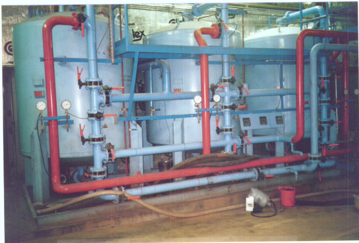
GRANULAR ACTIVATED CHARCOAL COLUMNS
