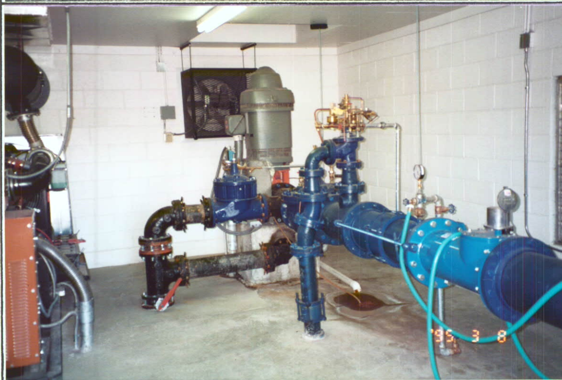
INSIDE OF PUMP HOUSE 125 HP PUMP
