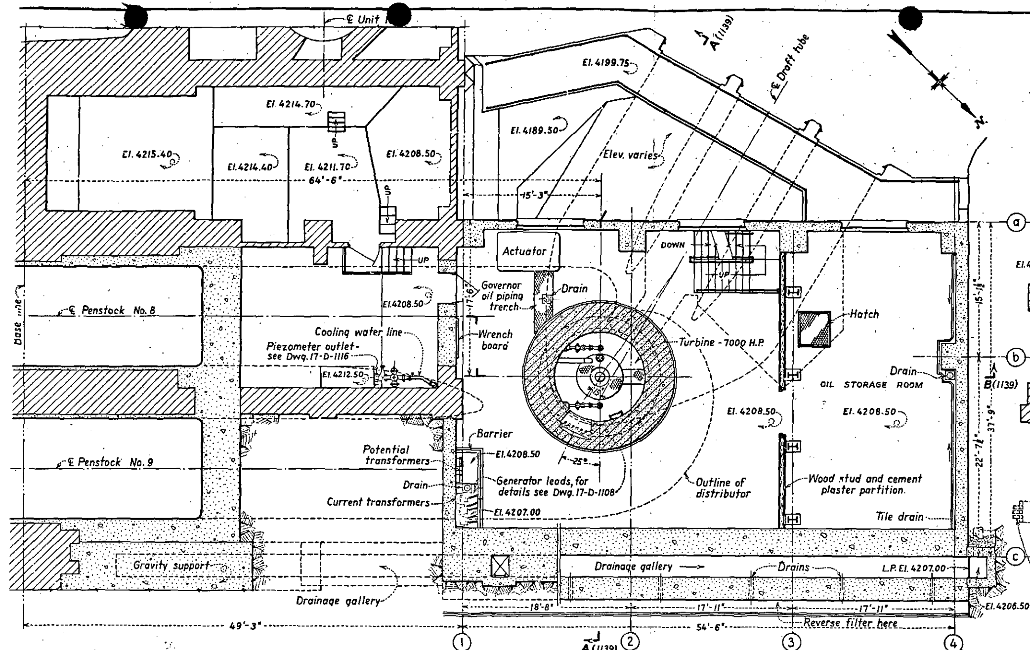
PLAN - FLOOR ELEV. 4208.50
