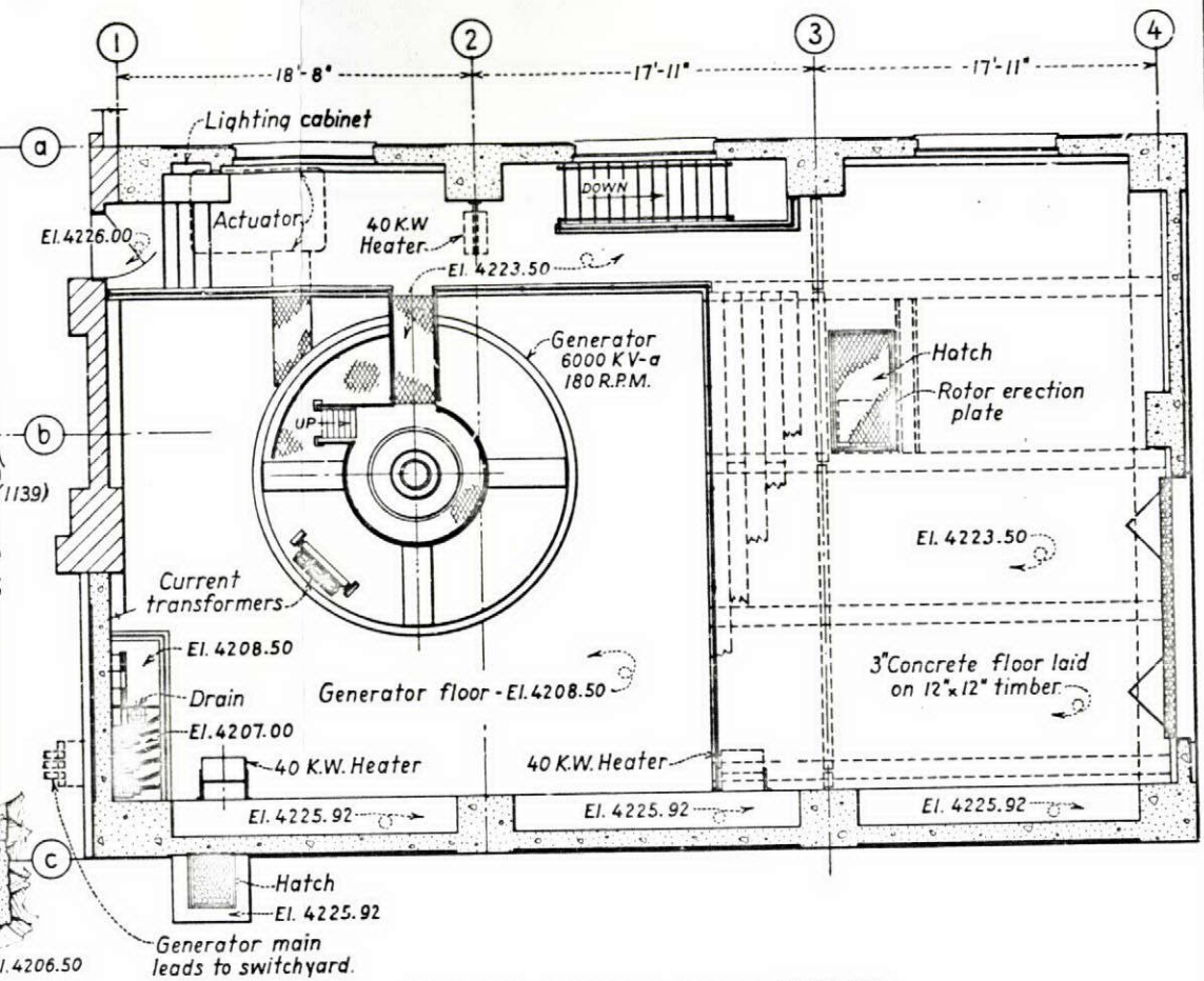
PLAN - FLOOR ELEV. 4223.50
