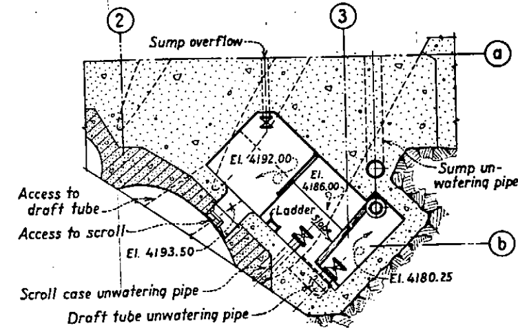
PLAN - FLOOR ELEV. 4197.00
