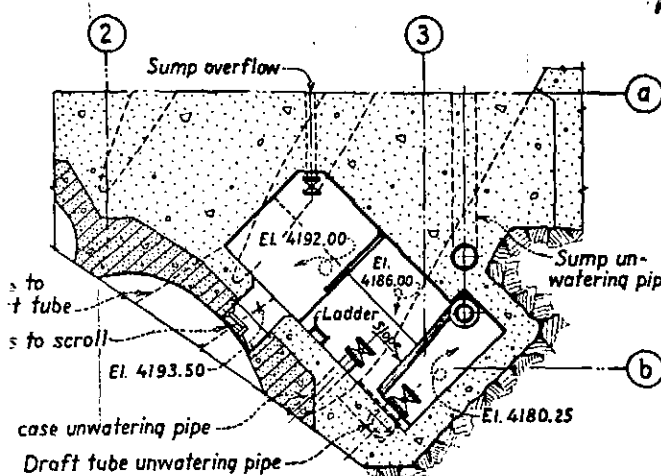
PLAN - FLOOR ELEV. 4197.00
