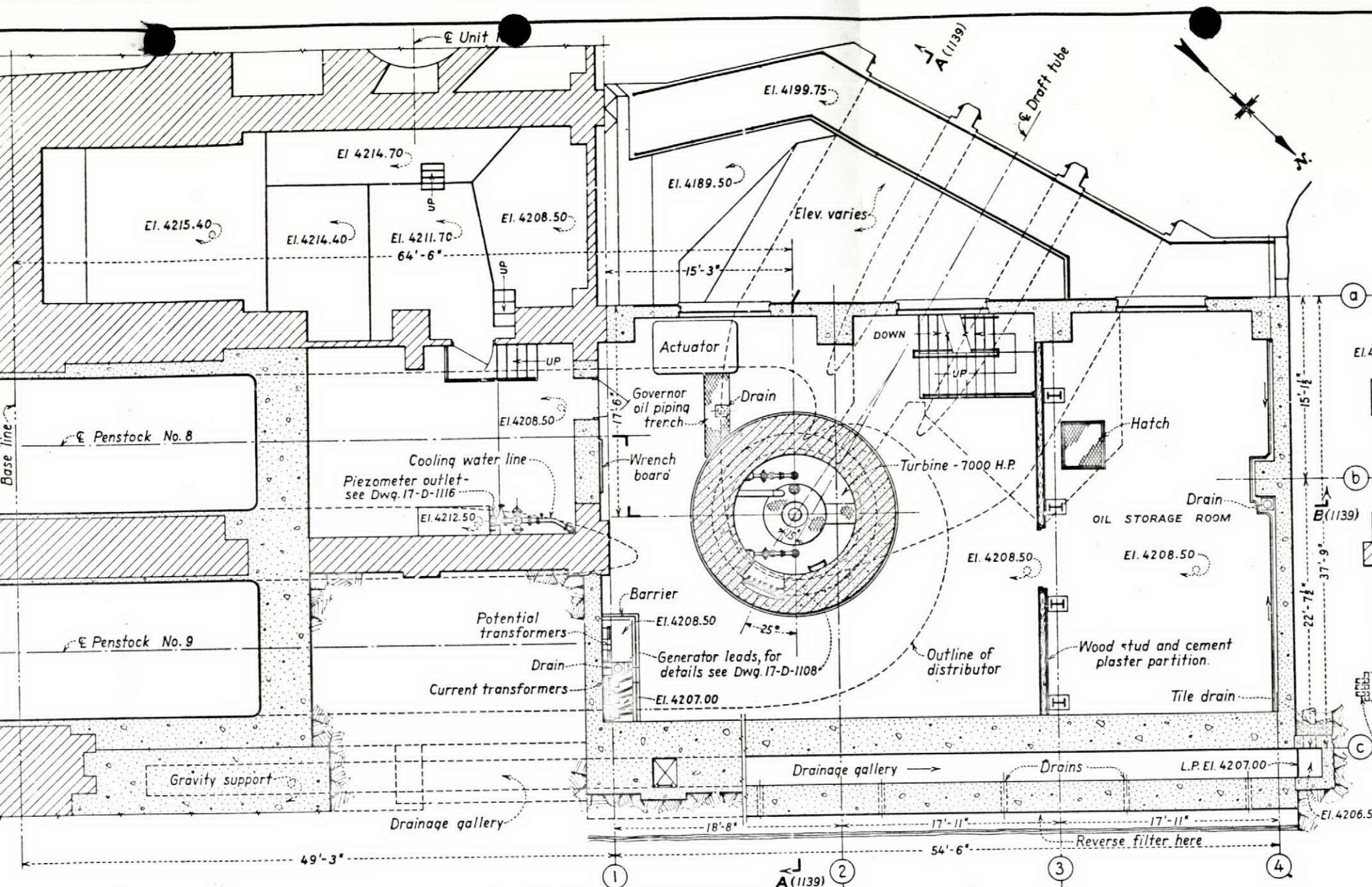
PLAN - FLOOR ELEV. 4208.50
