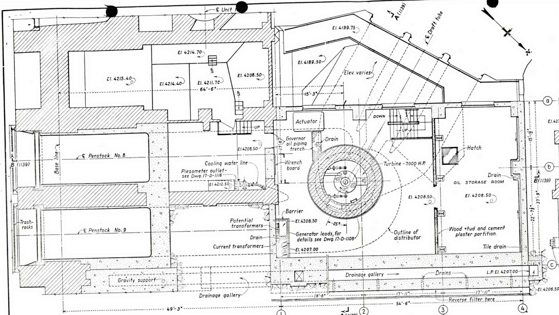
PLAN - FLOOR ELEV. 4208.50
