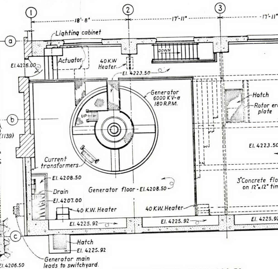
PLAN - FLOOR ELEV. 4223.50
