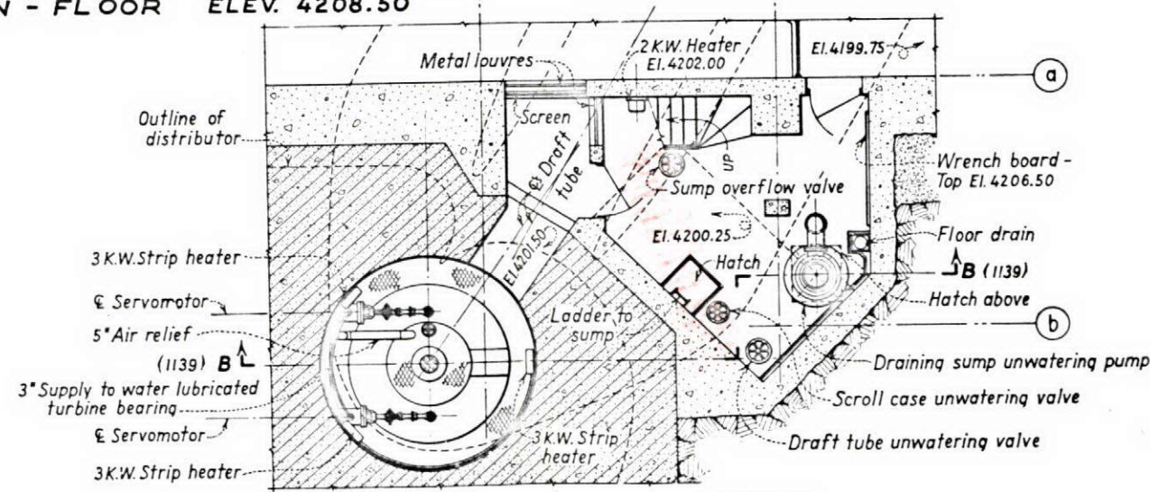
PLAN - FLOOR ELEV. 4200.25
