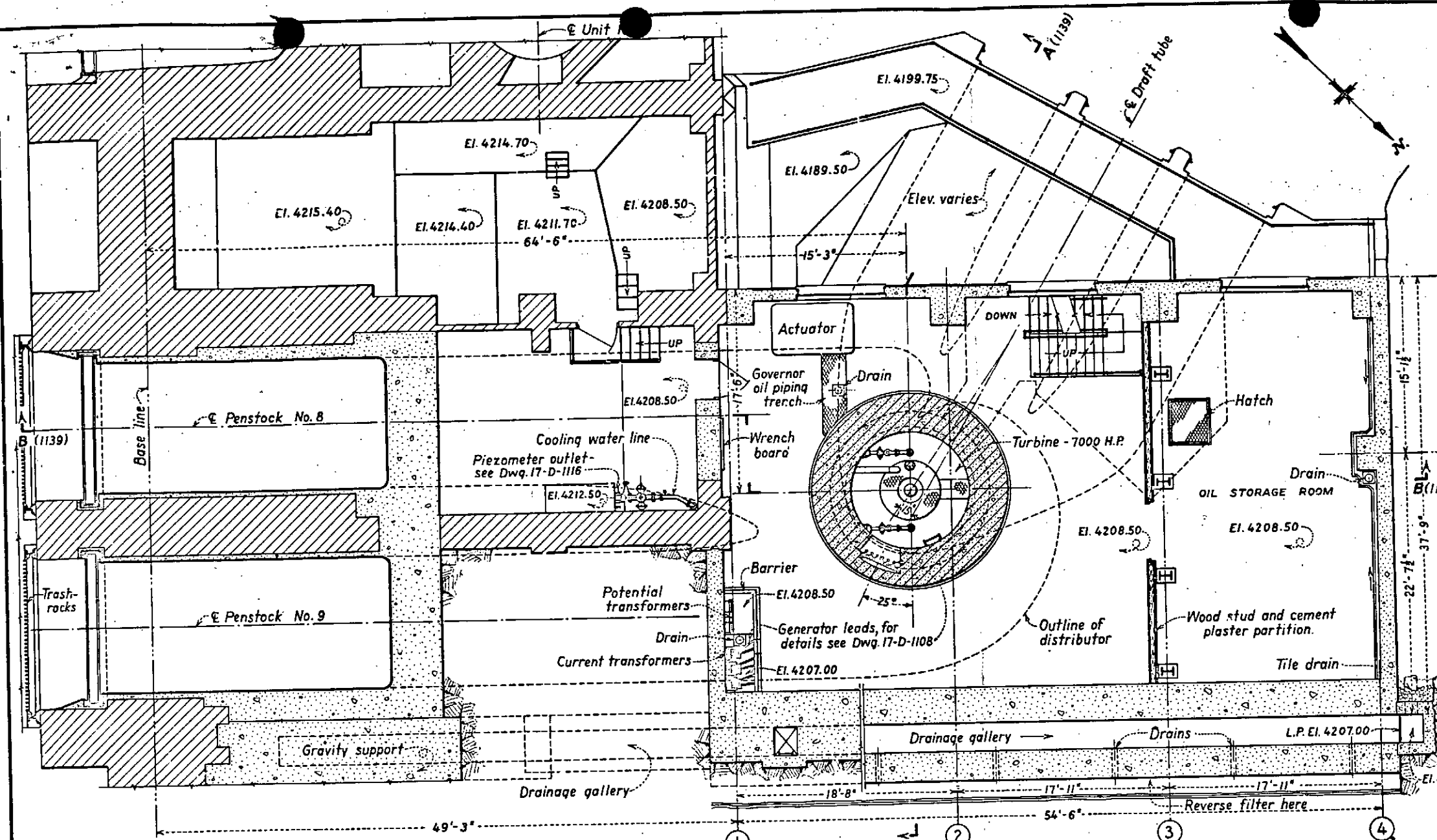
PLAN - FLOOR ELEV. 4208.50
