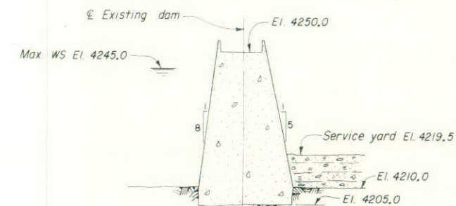
SECTION A CLOSURE SECTION
