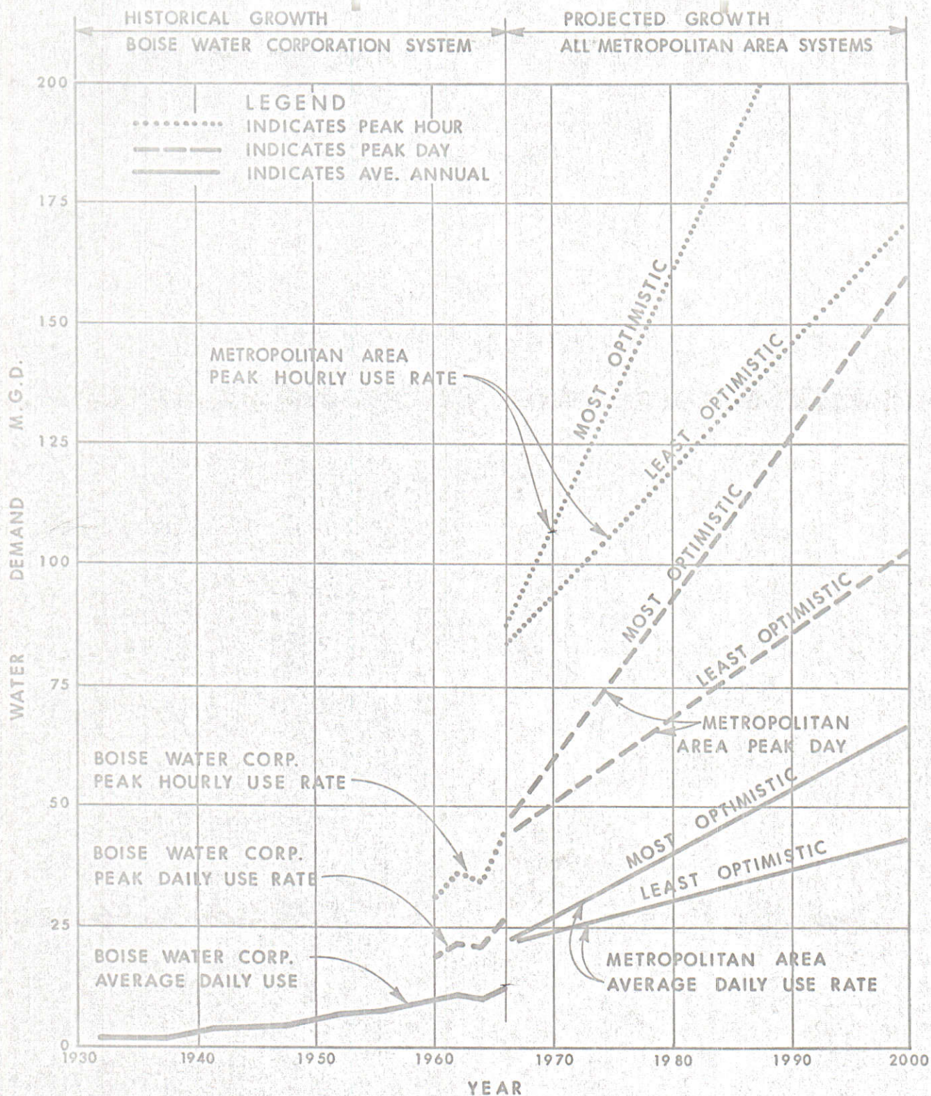
FIGURE 7 CITY OF BOISE, IDAHO METROPOLITAN AREA WATER STUDY WATER REQUIREMENTS BY YEARS
