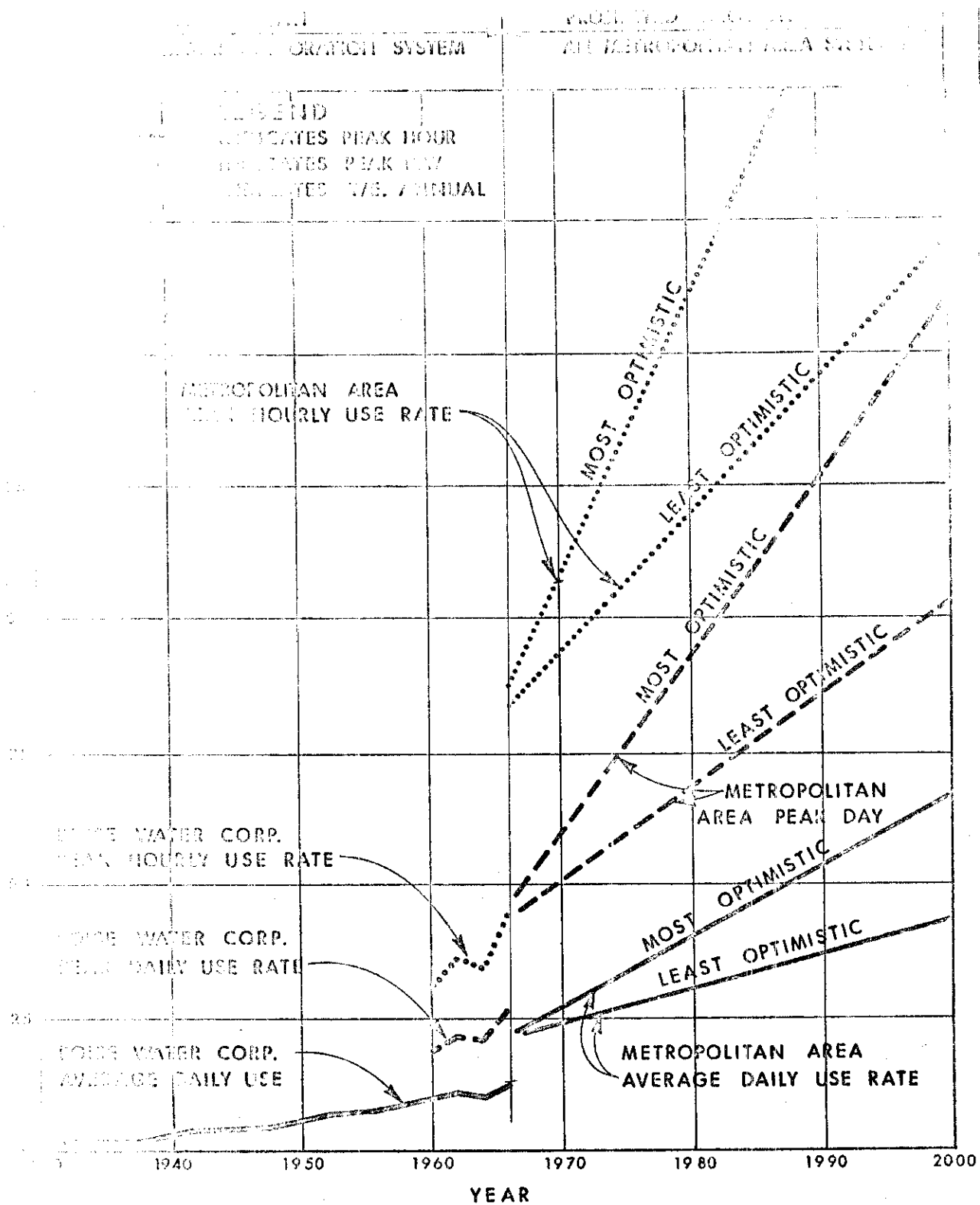
FIGURE 7 CITY OF BOISE, IDAHO METROPOLITAN AREA WATER STUDY WATER REQUIREMENTS BY YEARS
