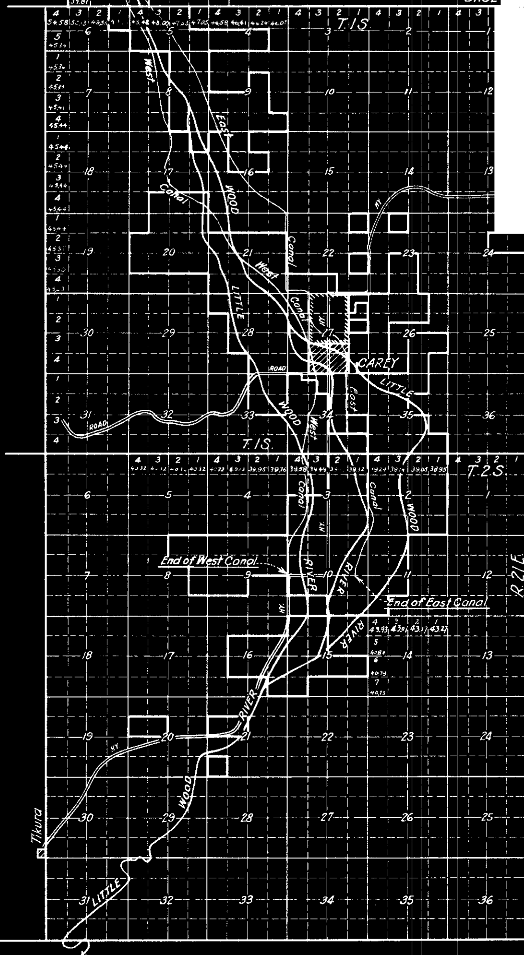
MAP OF LITTLE WOOD RIVER IRRIGATION DISTRICT Showing Boundary of District and Source of Water Supply BLAINE COUNTY-IDAHO Scale:- 1 Inch = 1 Mile Nov. - 1938 Compiled By Raymond J. Briggs Consulting Engineer, Boise, Idaho.
