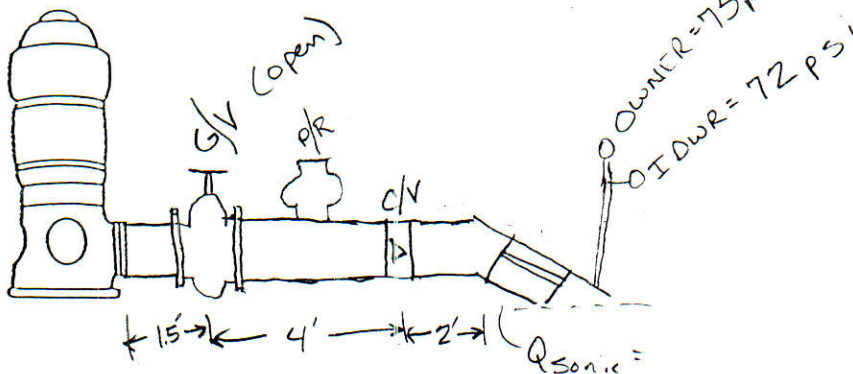
DIAGRAM OF PUMPING UNIT
