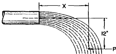
Figure 63. Rate of flow from a horizontal pipe can be estimated from the distance x .
