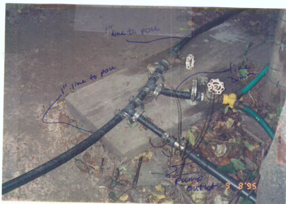
1.0 Hp Starite pump 1 1/2" intake 1" outlet outlet
