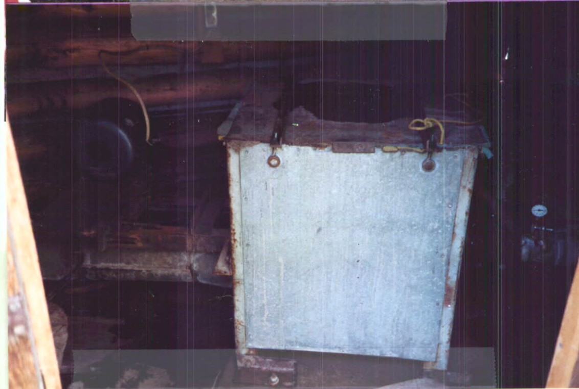
Pelton wheel Box AND Generator
