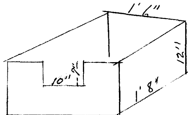
Headgate and Measuring Device on Miles Rice Diversion
