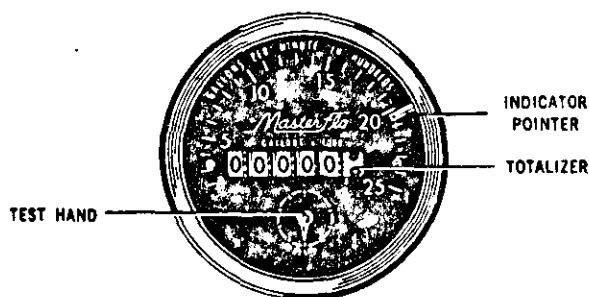
TYPICAL INDICATOR-TOTALIZER DIAL
