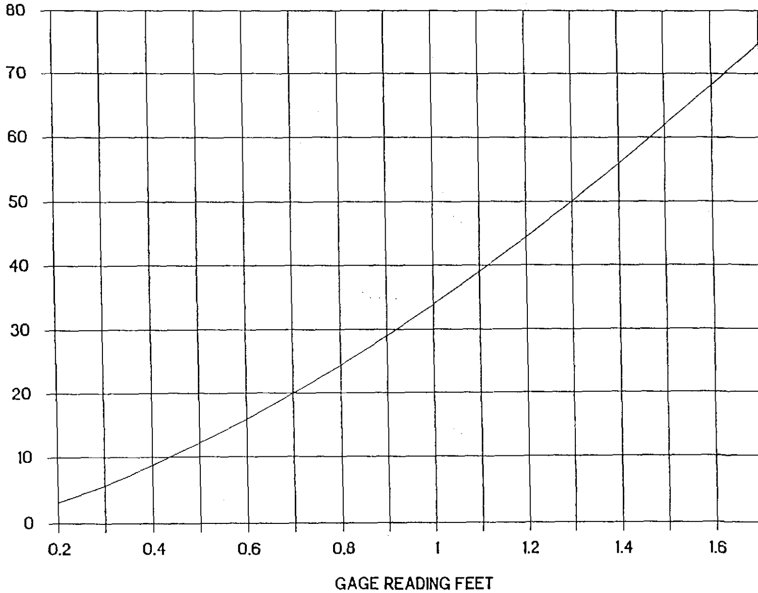
CLEAR SPRINGS 10 FT WEIR RATING CURVE
