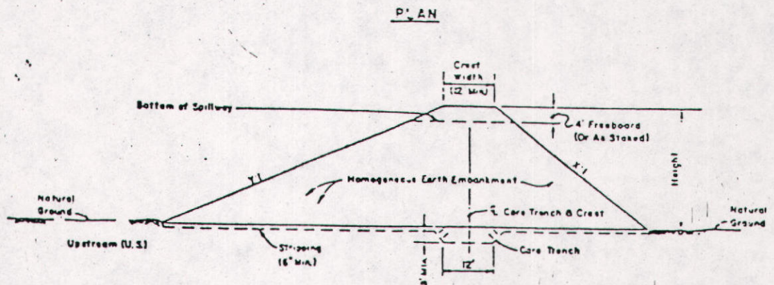
CROSS-SECTION (BOTTOM OF DRAINAGE)
