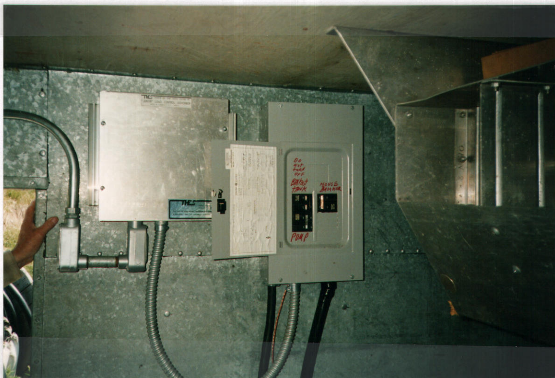
Fig. 5 - Control boxes for power supply inside powerhouse.
