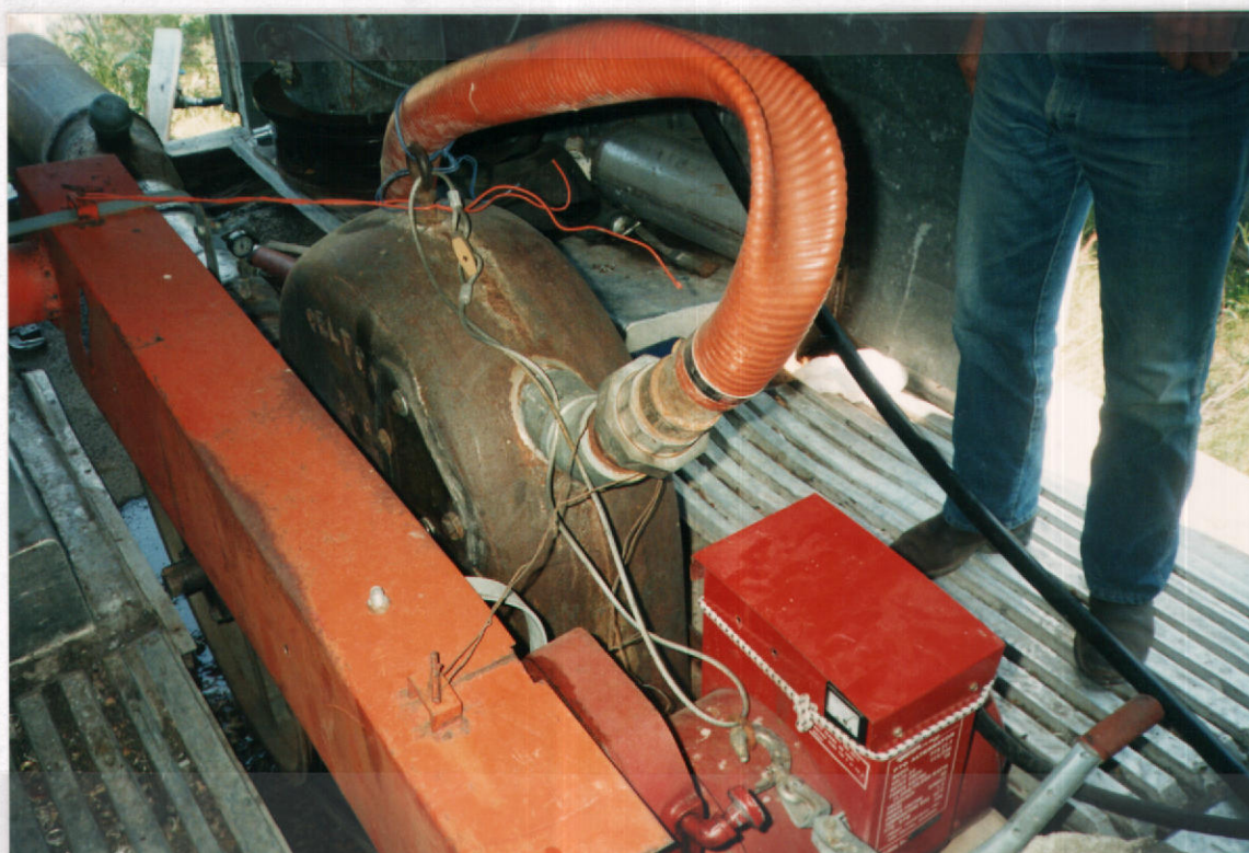
Fig. 3 - Inside of powerhouse showing Pelton Wheel and drive assembly.
