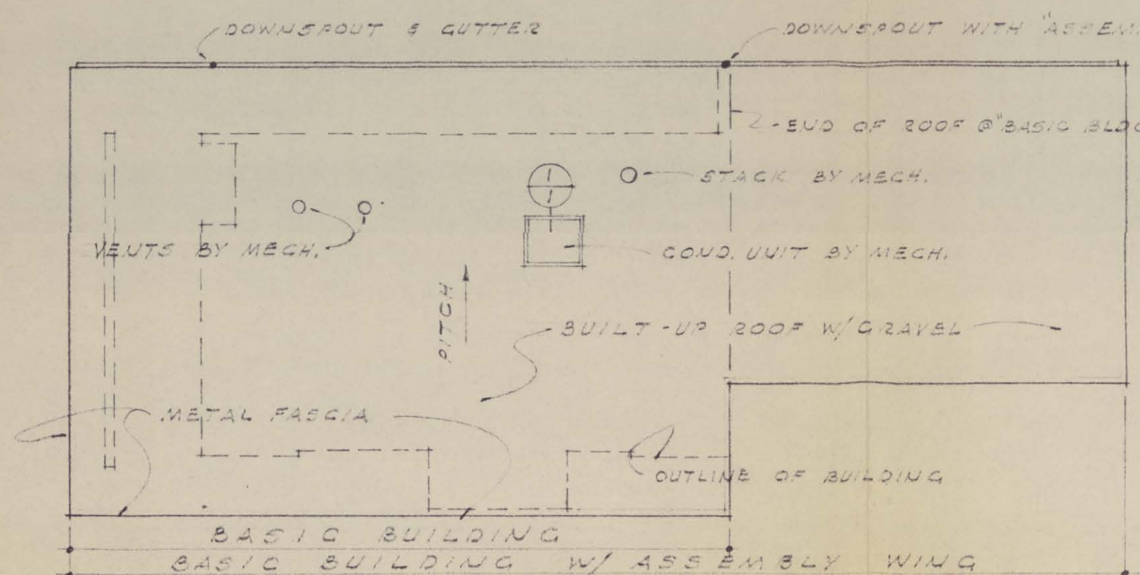
ROOF PLAN SCALE: 1/8" = 1'-0"
