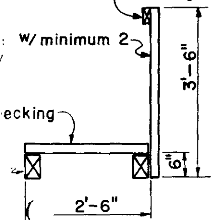
PEDESTRIAN BRIDGE SECTION BB Scale 1" = 2'
